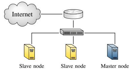
Figure 2. Example RPi configuration for example use cases of HCL
