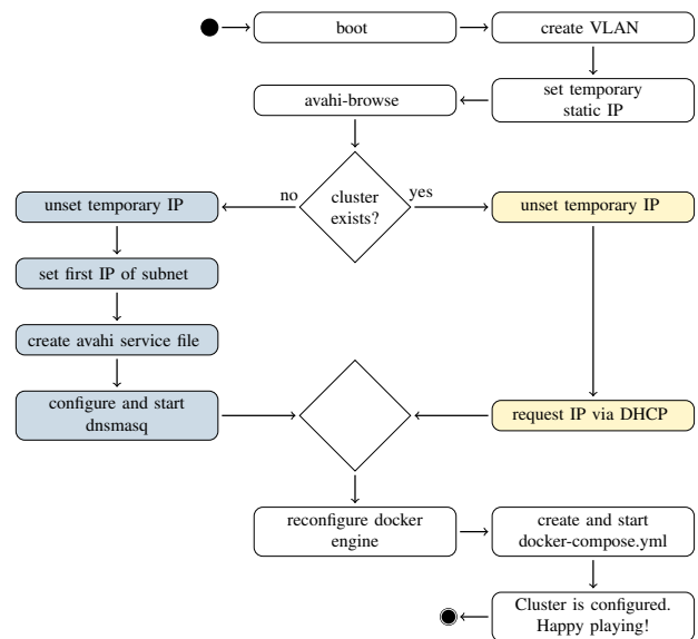
Figure 1. Activity Diagram of the node configuration of HCL. White activities occur on all nodes, while blue are associated with master nodes and yellow ones with slave nodes.
